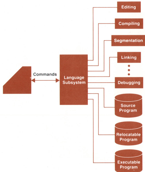
Fig. 2. HP 3000 program development is simplified by the language subsystem concept.
