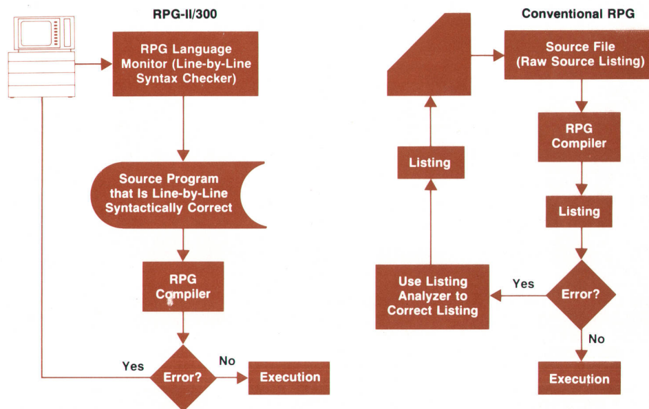
Fig. 6. RPG-II/300 and conventional RPG program development cycle.
